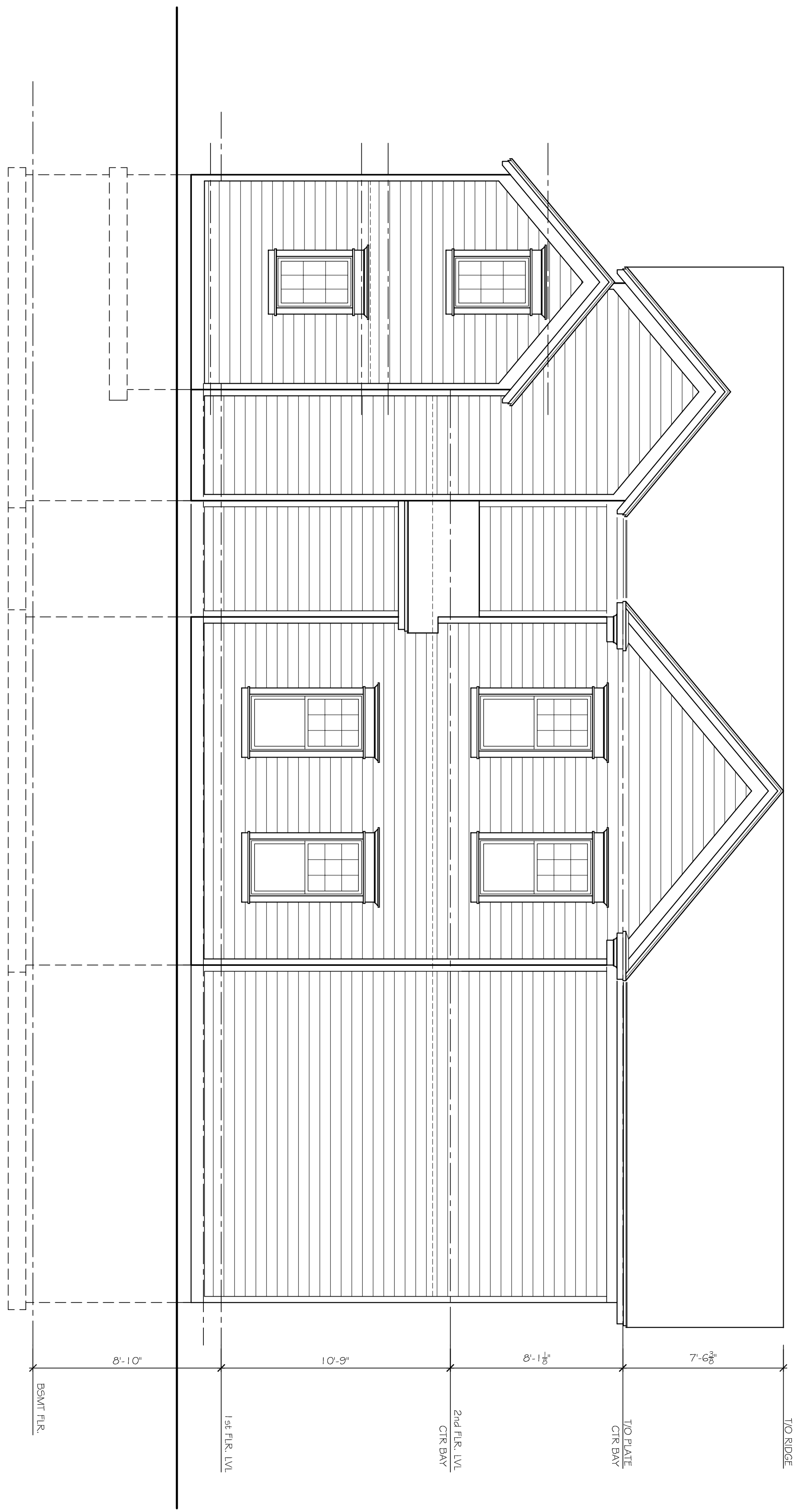
NORTH ELEVATION SCALE 1/4"=1'-0"
